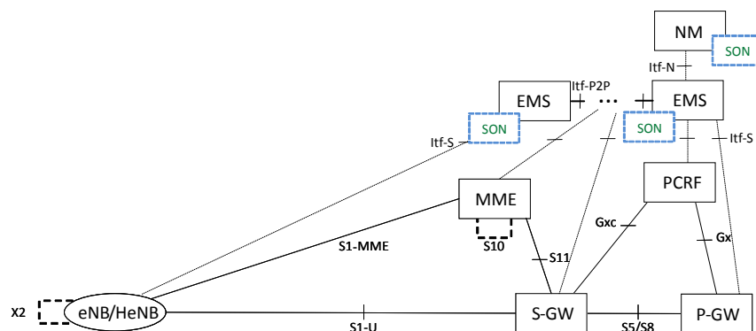
Figure 8 Centralized SON architecture
