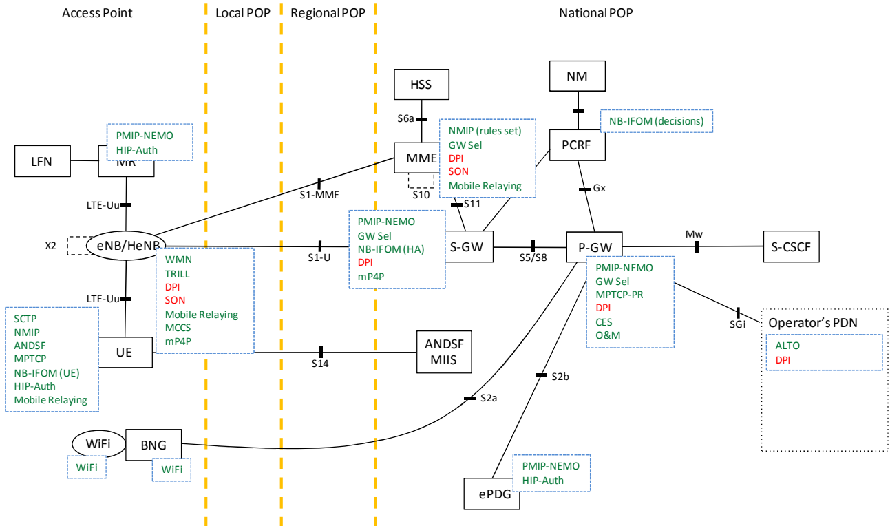
Figure 15. Centralized Architecture with all MEVICO technologies.
