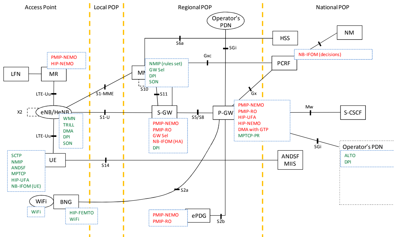
Figure 12 Distributed architecture with selected technologies
