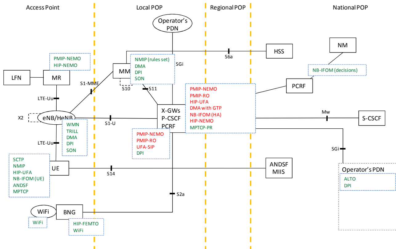
Figure 13 Flat architecture with selected technologies
